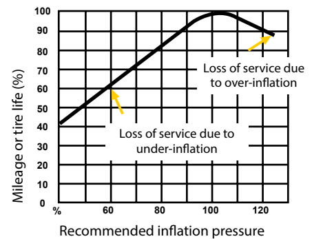
Effect of inflation pressure on tire life
